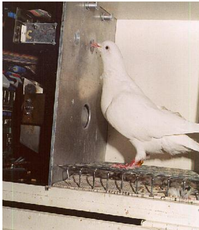
Skinner's box
